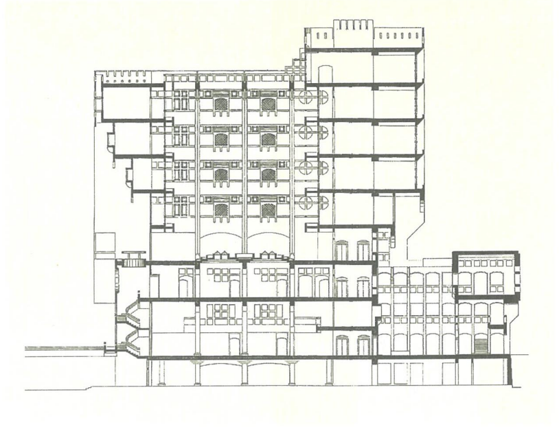
NORTH-SOUTH SECTION
