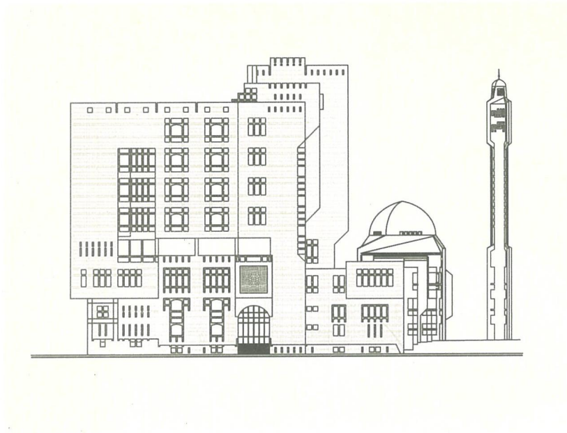
EAST ELEVATION
