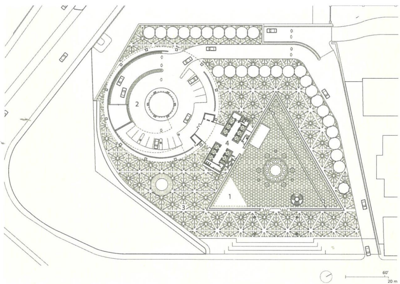
SITE PLAN
