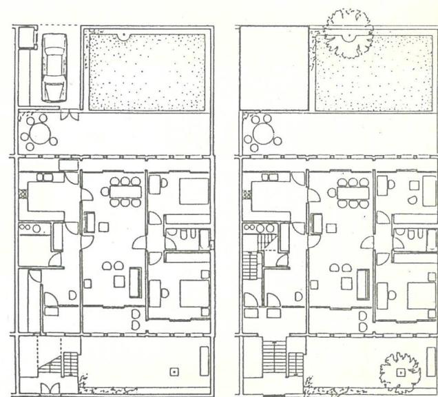
TYPICAL APARTMENT PLAN
